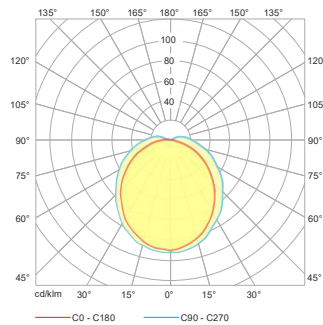
Diffused Beam
