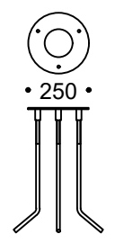
Anchorage Detail
