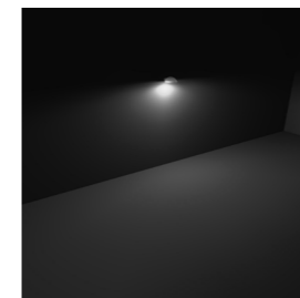
M3 degree
